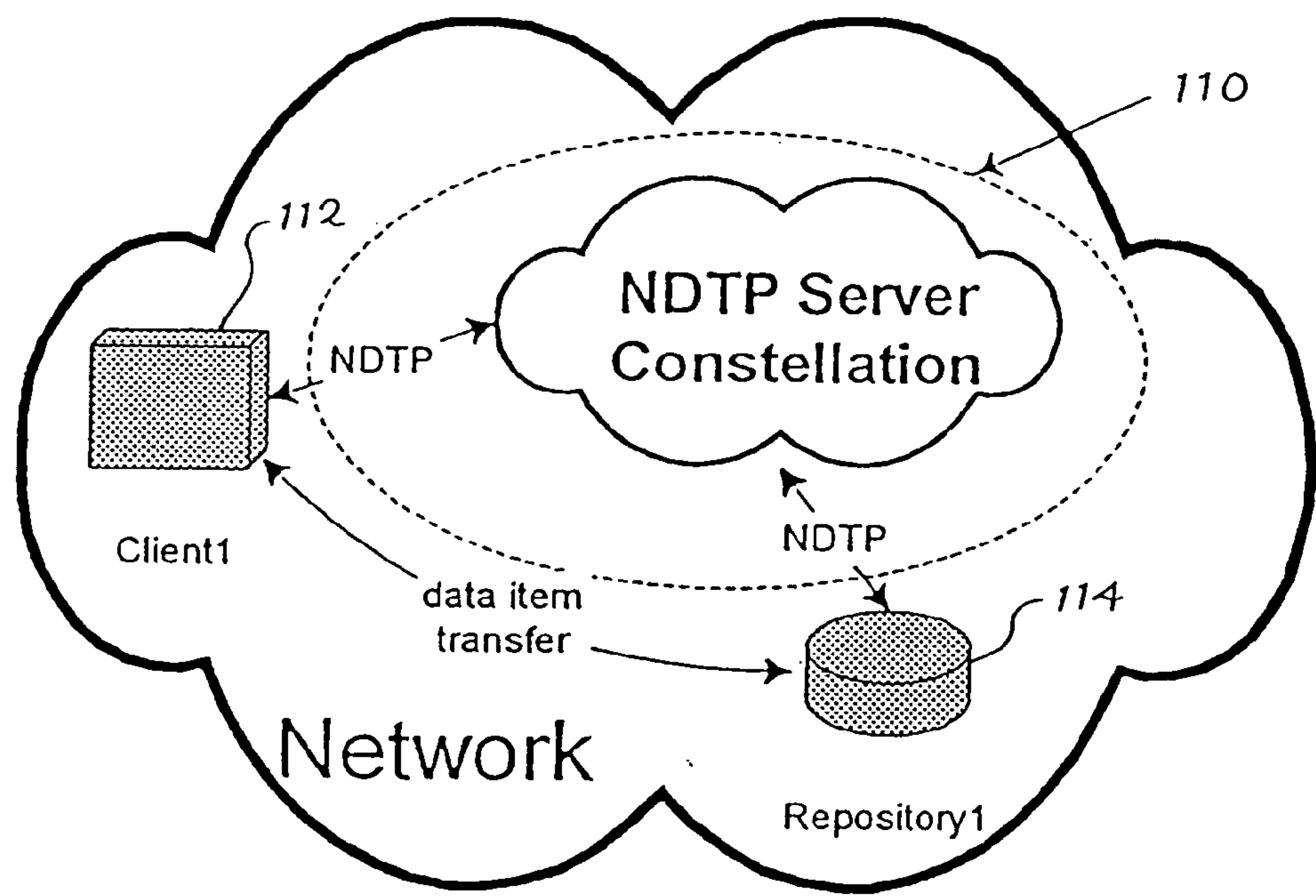
Fig. 11 NDTP Server Constellation Context
