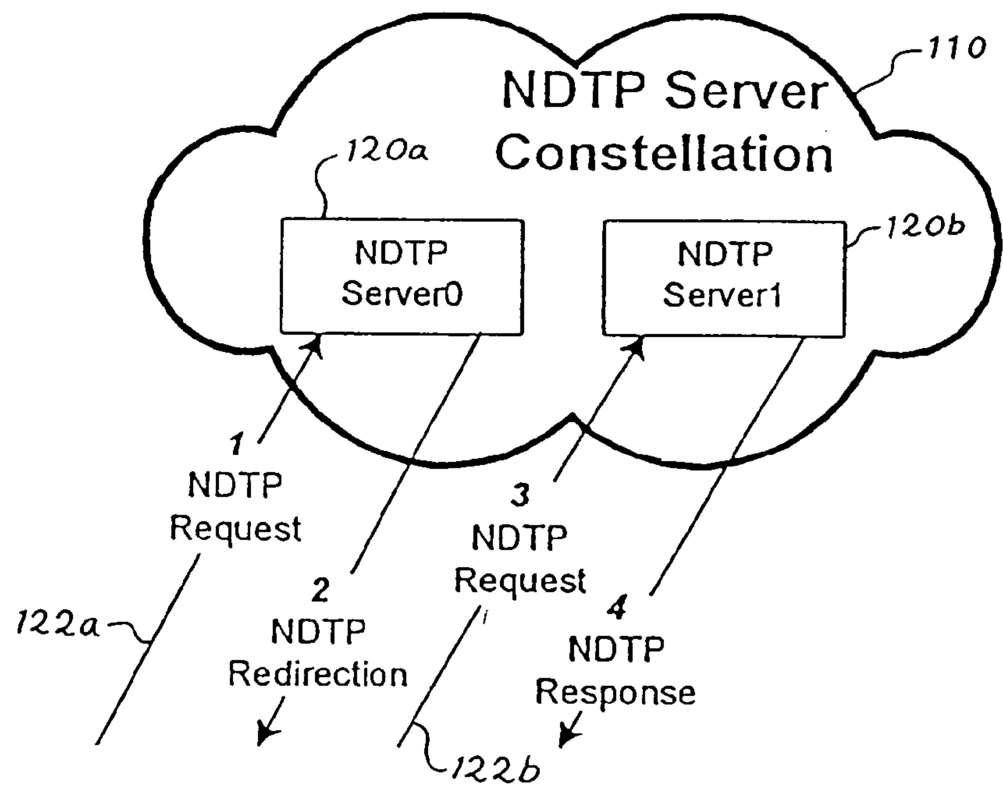
Fig. 12 NDTP Client-Centric Constellation
